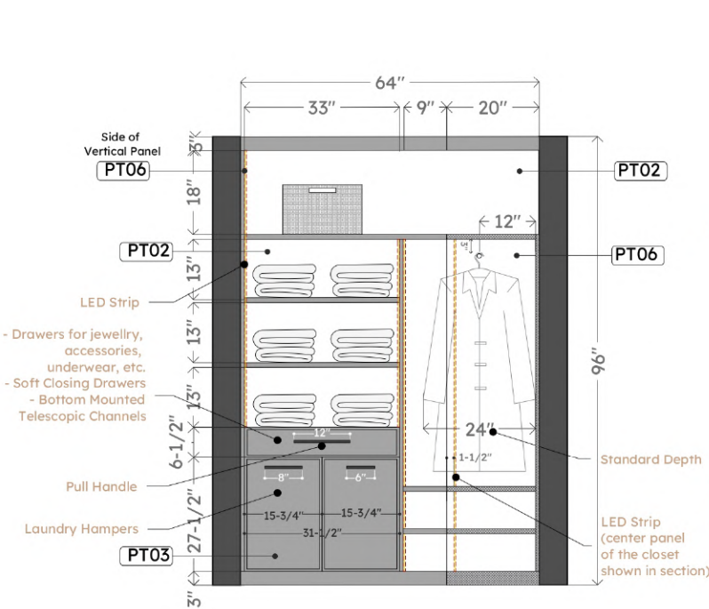
1 Cross Section I- 313 Scale 3/4" = 0" 1'
