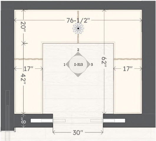
A-106 Primary Bedroom Walk-in Closet Floor Plan Detail Scale 3/4" = 0" 1'
