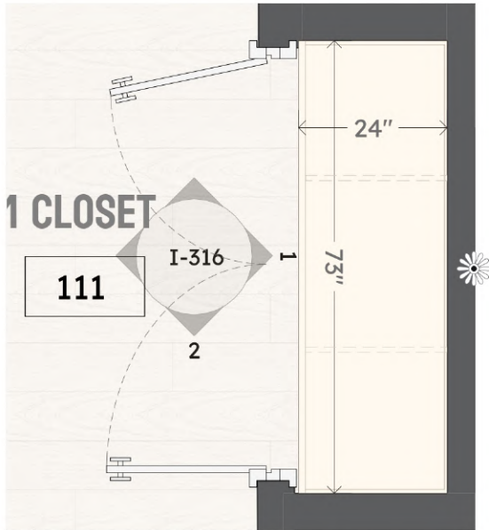
A-111 Guest Bedroom Closet Floor Plan Detail Scale 1" = 0" 1'
