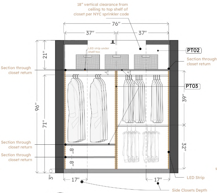
2 Elevation-Section I- 313 Scale 3/4" = 0" 1'
