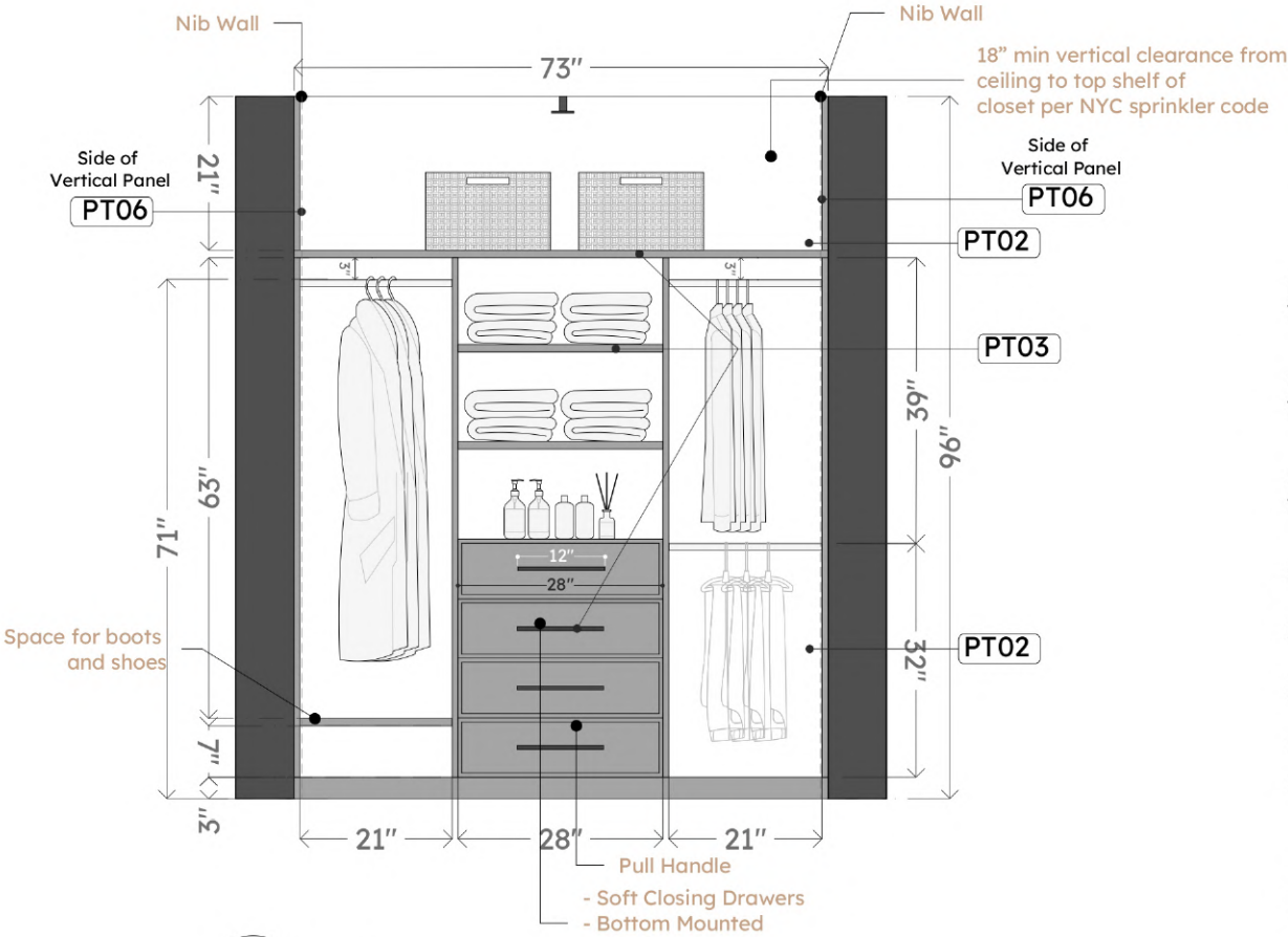
1 Front Elevation I- 316 Scale 1" = 0" 1'
