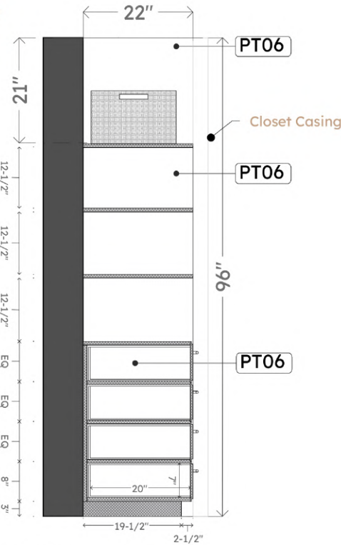
2 Section I- 316 Scale 1" = 0" 1'
